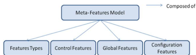
Fig. 1 Meta-features Model
