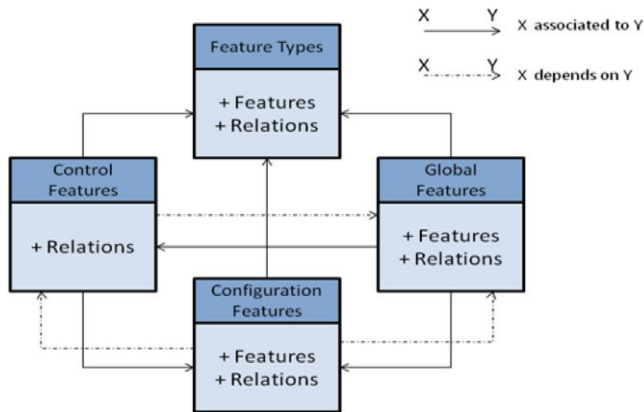
Fig. 2 Meta-features connections
